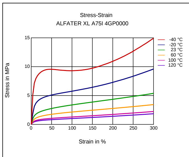
Stress-Strain
